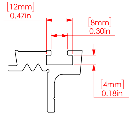
T-SLOT DETAIL ACCEPTS STANDARD 1/4" OR M6 HEX BOLTS
